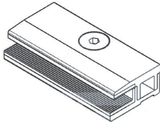
Figure 2: Hilti End Clip
